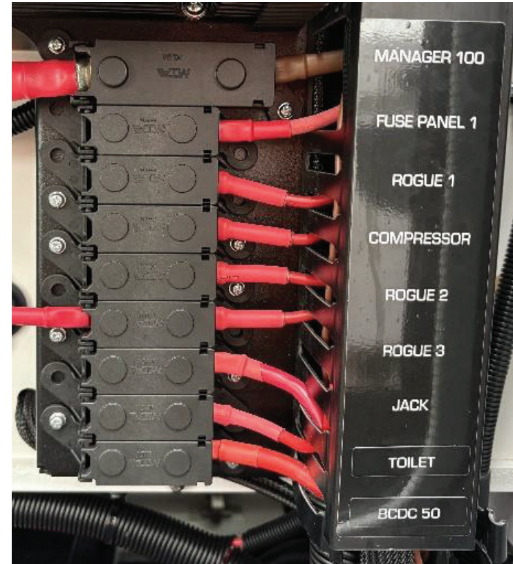
System Supply Fuses – Bottom right corner of the electrical panel
